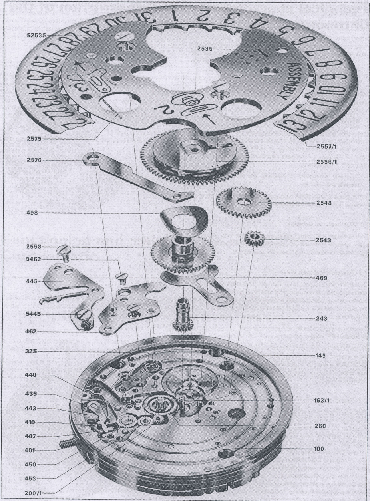
EXPLODED VIEW OF THE MOVEMENT ON THE CALENDAR SIDE
